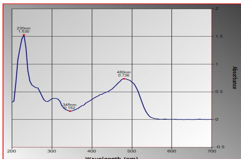
Fig SM12. UV- Vis Spectrum of Sulphanilamide and 2-Naphthol in methanol
