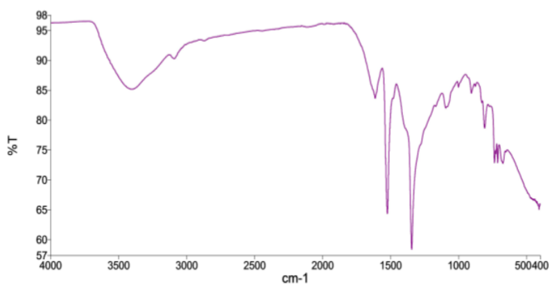
Fig. SM28. Infra Red spectrum of 3-Nitroaniline and Catechol
