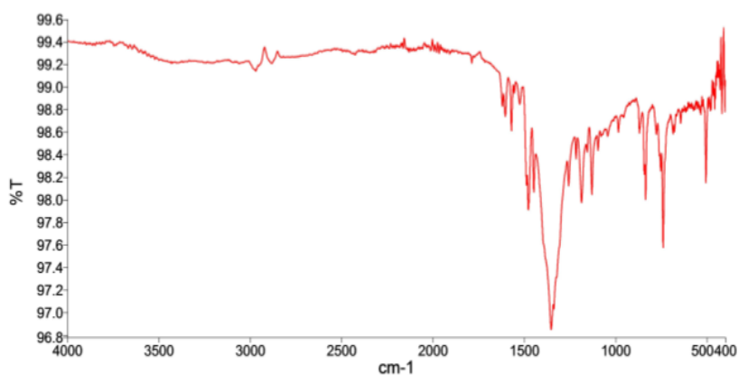
Fig. SM16. Infra-red spectrum of 2-Nitroaniline and 2-Naphthol
