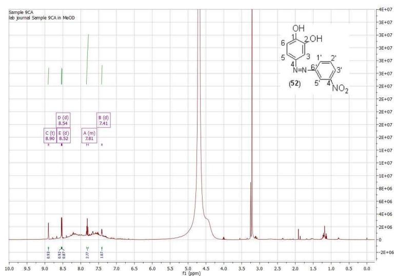
Fig SM29. 1 H NMR spectrum of 3-Nitroaniline and Catechol
