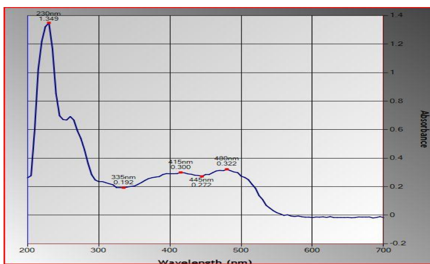
Fig.SM8. UV- Vis Spectrum of 4-Chloroaniline and 2-Naphthol in methanol
