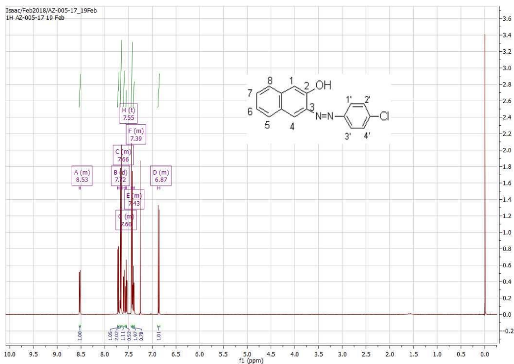
Fig.SM10. 1 H NMR of 4-Chloroaniline and 2-Naphthol
