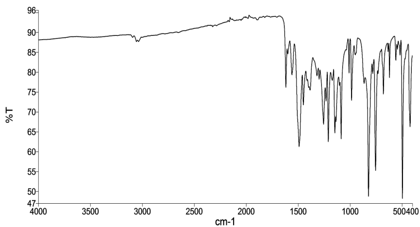
Fig. SM9. Infra Red spectrum of 4-Chloroaniline and 2-Naphthol
