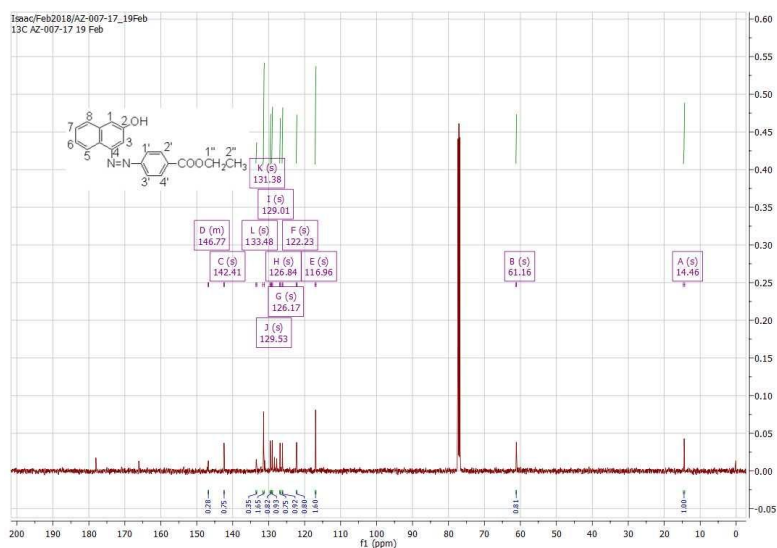
Fig SM7. 13 C NMR spectrum of Ethyl-aminobenzoate and 2-Naphthol
