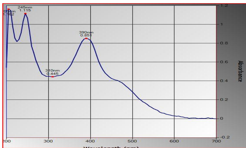
Fig. SM27. UV- Vis Spectrum of 3-Nitroaniline and Catechol in methanol
