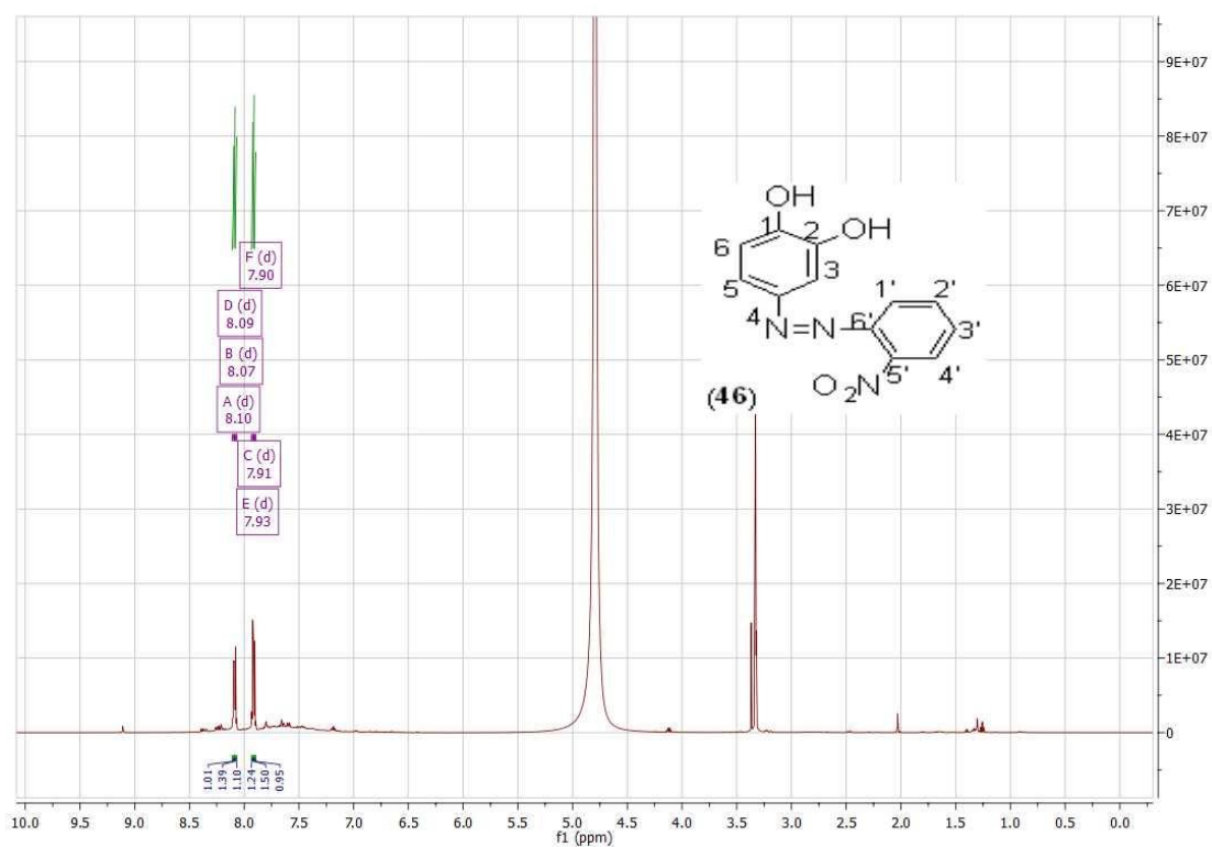
Fig. SM20. 1 H NMR spectrum of 2-Nitroaniline and Catechol
