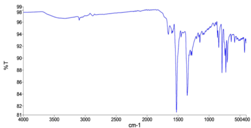
Fig. SM22. Infra Red spectrum of 2-Nitroaniline and Quinol
