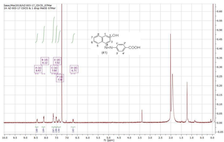
Fig. SM3. 1 H NMR spectrum of p -aminobenzoic acid and 2-Naphthol
