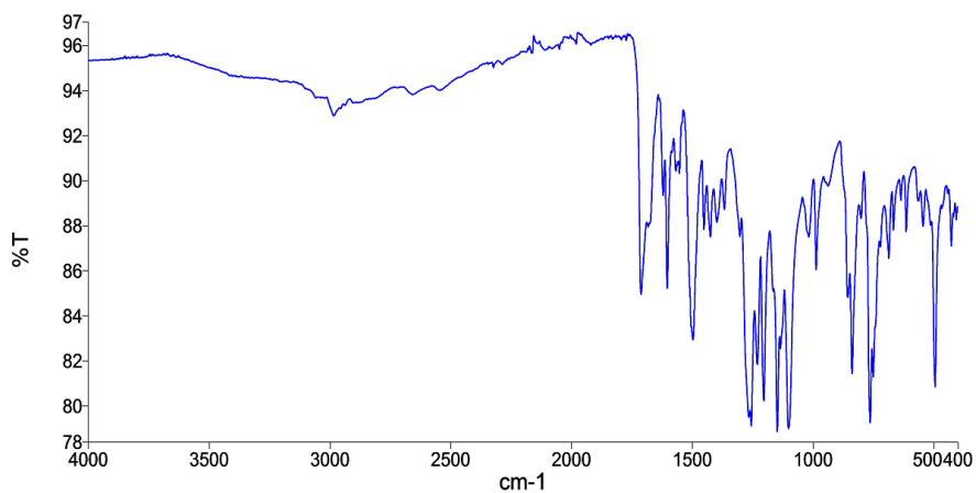
Fig. SM5. Infra-Red spectrum of Ethyl-aminobenzoate and 2-Naphthol
