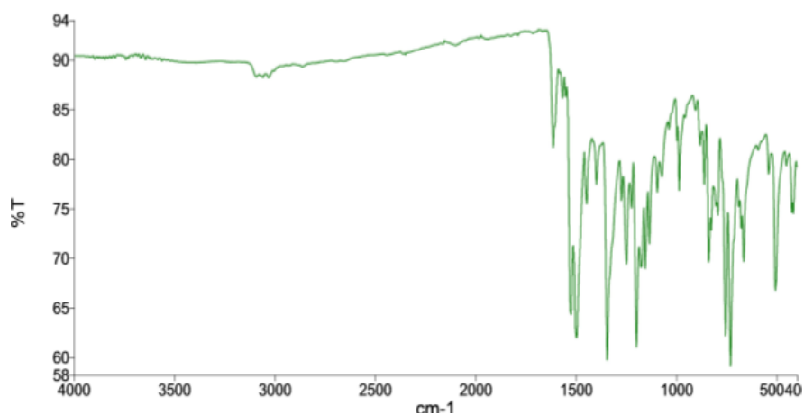
Fig. SM25. Infra Red spectrum of 3-Nitroaniline and 2-Naphthol
