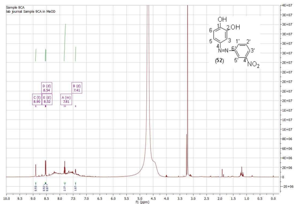
Fig. SM32. 1 H NMR spectrum of 3-Nitroaniline and Quinol
