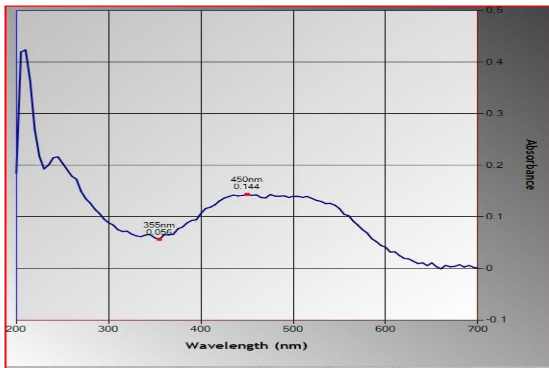
Fig. SM21. UV- Vis Spectrum of 2-Nitroaniline and Quinol in methanol
