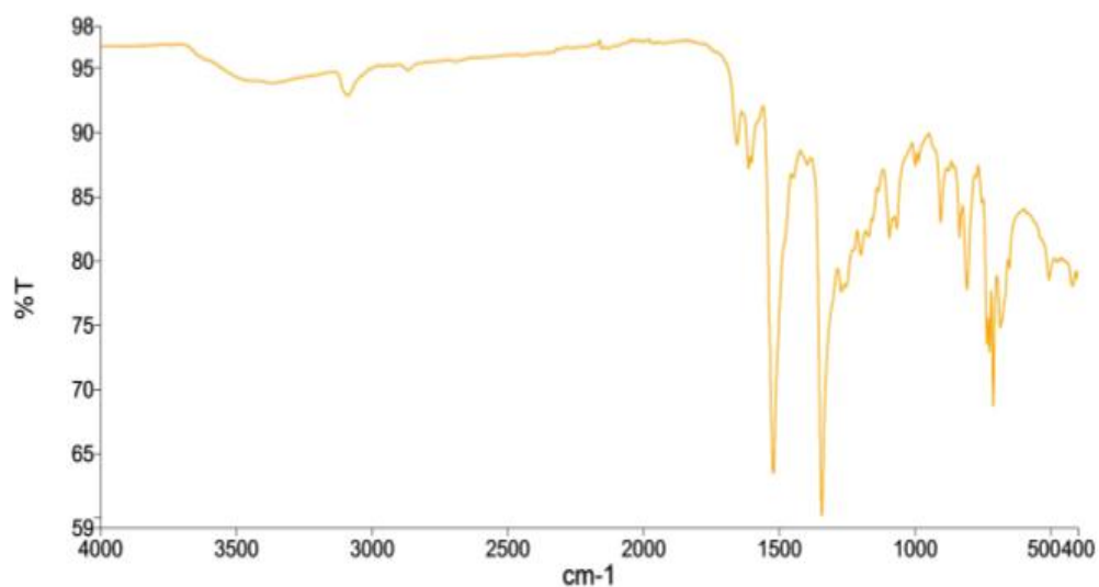
Fig. SM31. Infra Red spectrum of 3-Nitroaniline and Quinol
