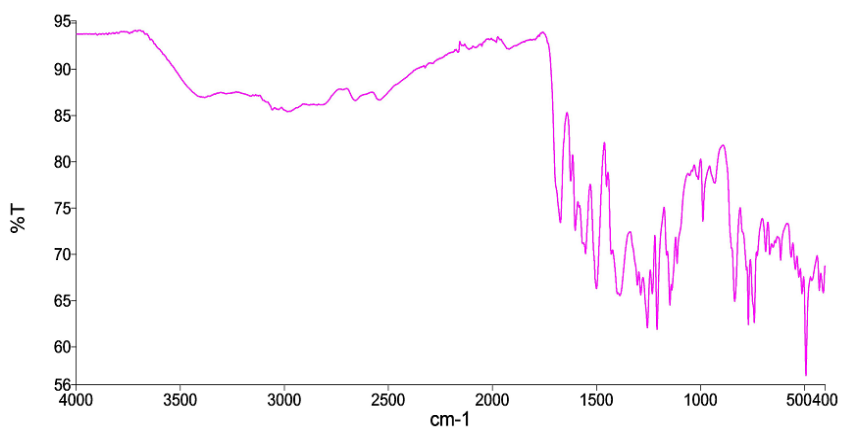
Fig. SM2. Infra red spectrum of p -aminobenzoic acid and 2-Naphthol
