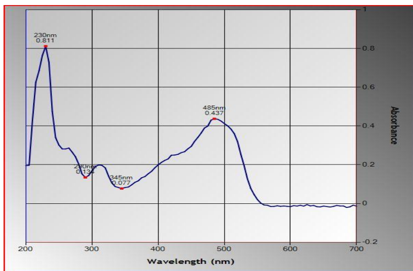
Fig. SM1. Spectra Data for p -aminobenzoic acid and 2-Naphthol (Compound 1)
