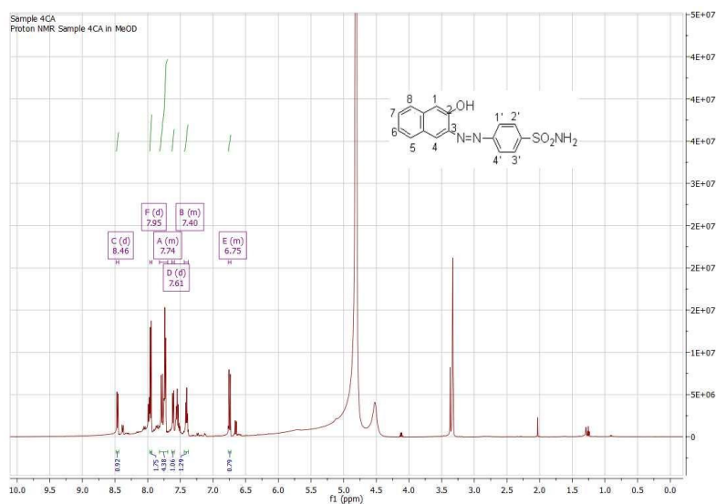
Fig. SM14. 1 H NMR spectrum of Sulphanilamide and 2-Naphthol
