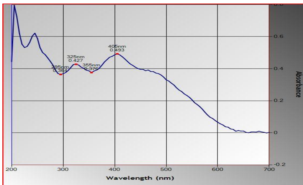
Fig. SM18. UV- Vis Spectrum of 2-Nitroaniline and Catechol in methanol
