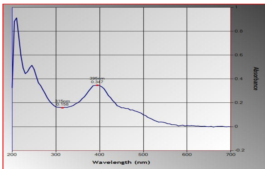
Fig SM24. UV- Vis Spectrum of 3-Nitroaniline and 2-Naphthol in methanol
