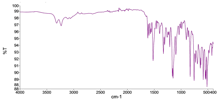
Fig. SM13. Infra Red spectrum of Sulphanilamide and 2-Naphthol
