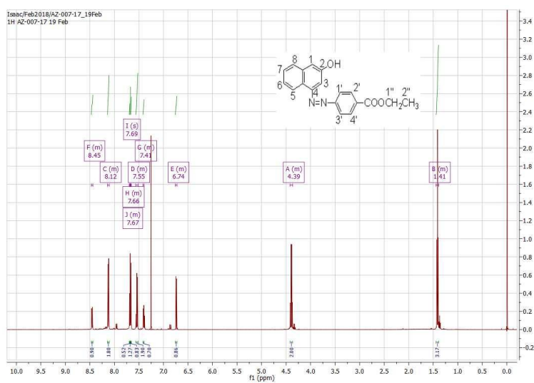
Fig. SM6. 1 H NMR spectrum of Ethyl-aminobenzoate and 2-Naphthol
