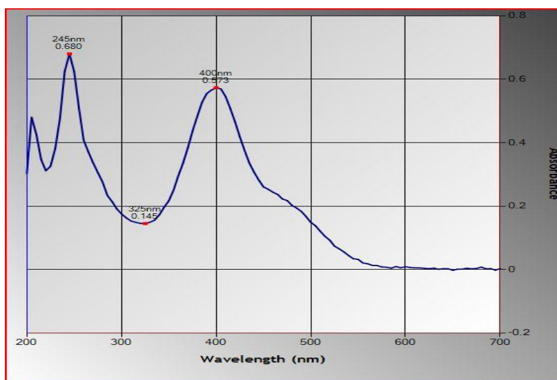
Fig. SM15. UV- Vis Spectrum of 2-Nitroaniline and 2-Naphthol in methanol
