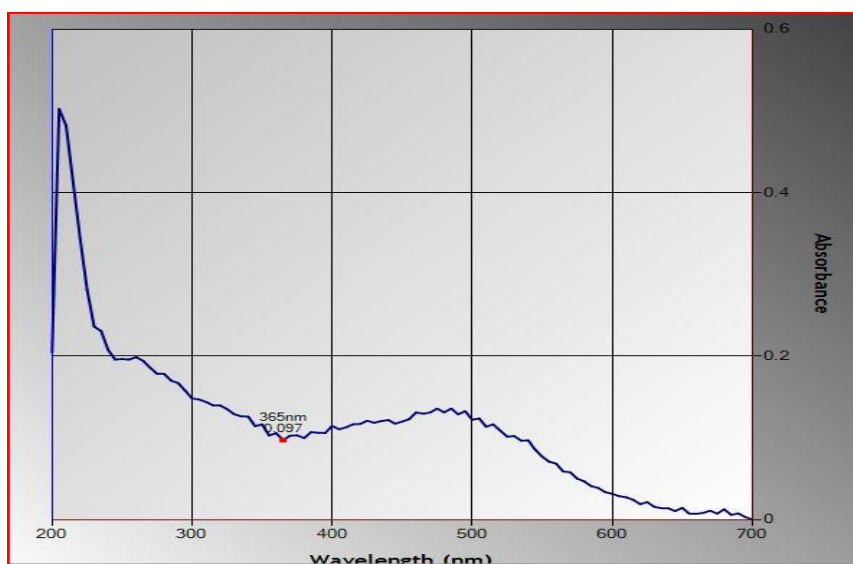
Fig. SM30. UV- Vis Spectrum of 3-Nitroaniline and Quinol in methanol
