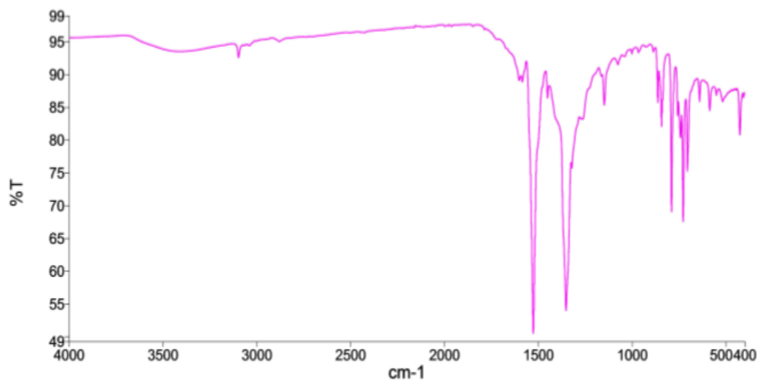
Fig. SM19. Infra Red spectrum of 2-Nitroaniline and Catechol
