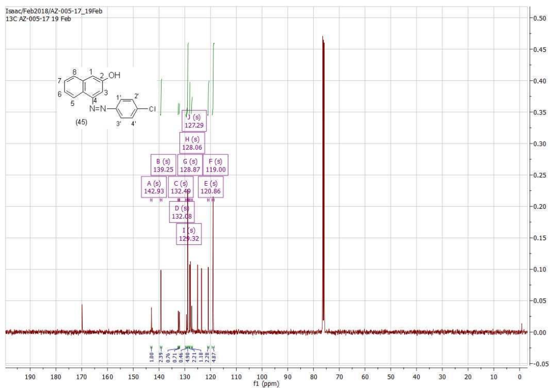
Fig.SM11. 13 C NMR spectrum of 4-Chloroaniline and 2-Naphthol
