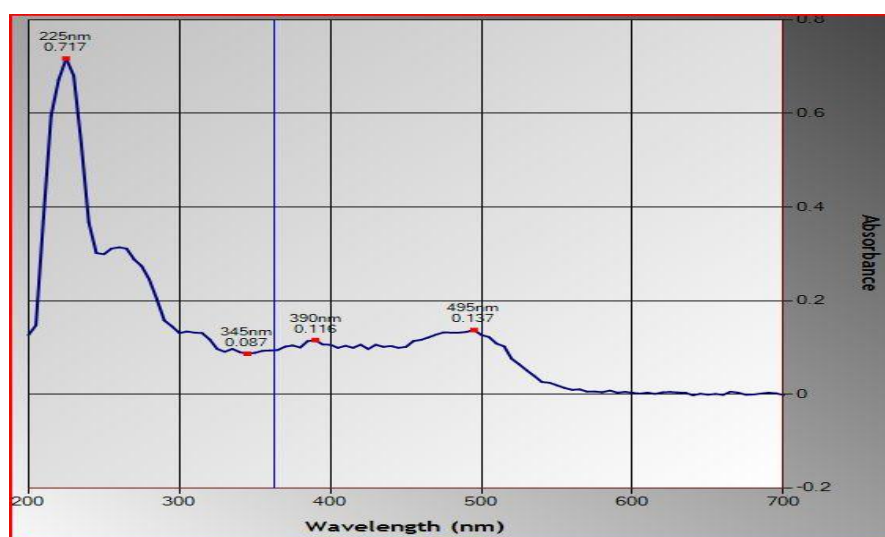
Fig. SM4. UV- Vis Spectrum of Ethyl-aminobenzoate and 2-Naphthol in methanol
