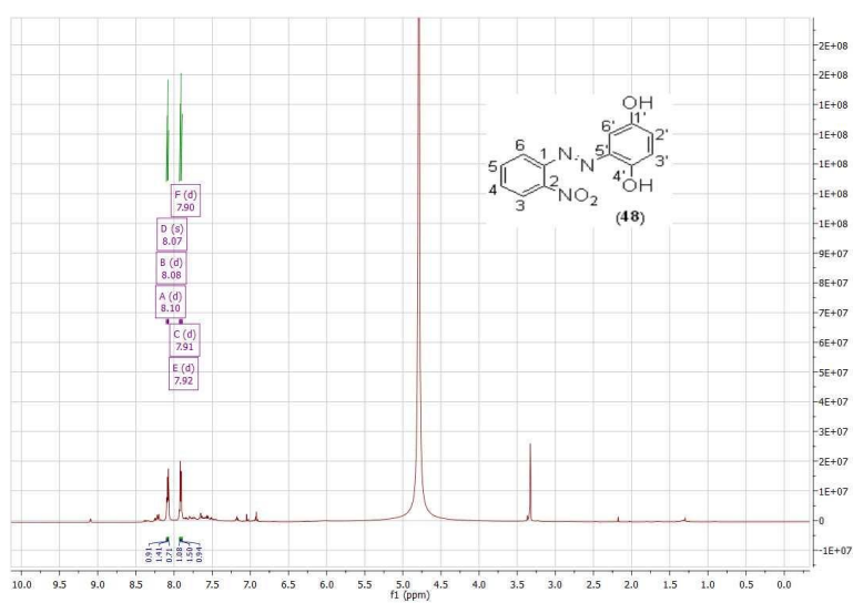
Fig SM23. 1 H NMR spectrum of 2-Nitroaniline and Quinol
